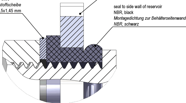
DETAILA (2 : 1)
