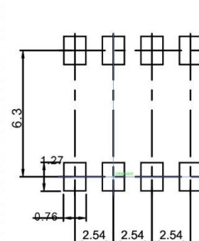
SOP8 (Top View)
