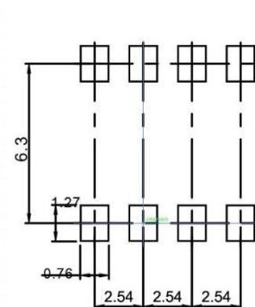
SOP8 (Top View)
